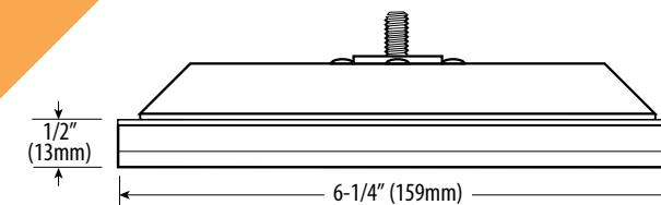
Backing plate: 43-148DAR
